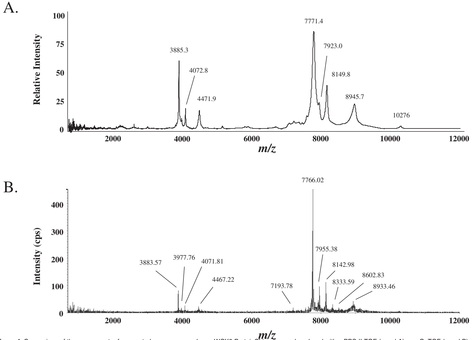
Figure 1 Comparison of the mass spectra from control serum prepared on a WCX2 ProteinChip array and analyzed with a PBS-II TOF (panel A) or a QqTOF (panel B) mass spectrometer.
