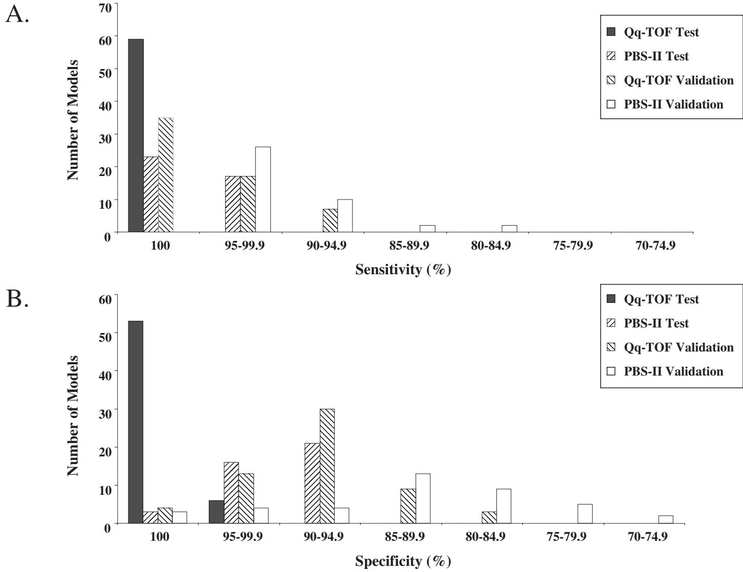
Figure 2 Histograms representing the testing and blinded validation results of sensitivity (A) and specificity (B) of the 108 models for MS data acquired on either a QqTOF or a PBS-II TOF mass spectrometer.
