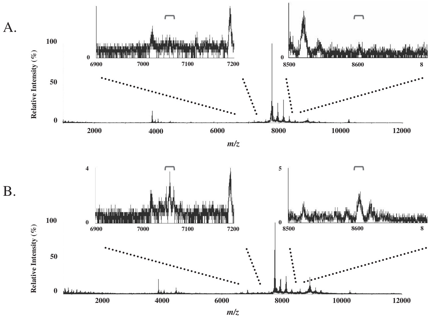
Figure 4 Comparison of SELDI QqTOF mass spectra of serum from an unaffected individual (A) and an ovarian cancer patient (B). Insets show expanded m/z regions highlighting significant intensity differences of the peaks in the m/z bins 7060.121 and 8605.678 (indicated by brackets) identified by the algorithm as belonging to the optimum discriminatory pattern.
